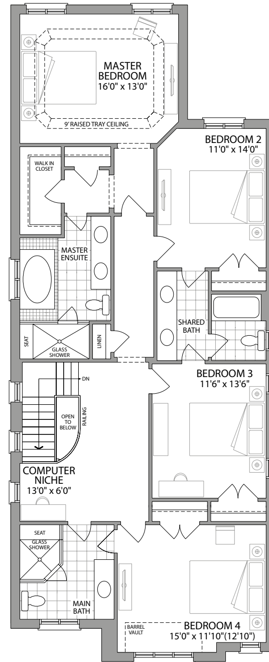
SECOND FLOOR
